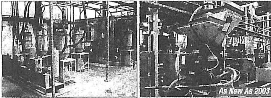
MAGUIRE GRAVIMETRIC BLENDERS
