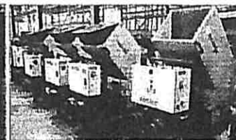
PARTIAL VIEW OF 48 ASSORTED GRANULATORS
