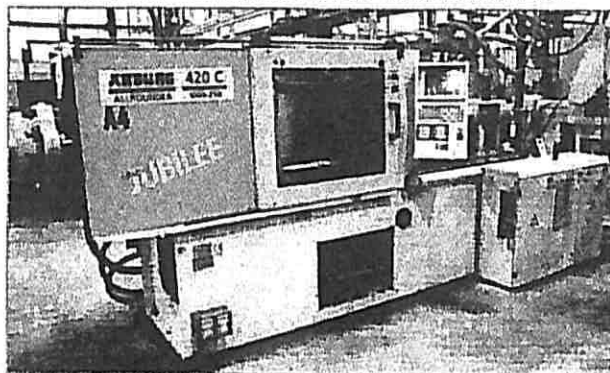
ARBURG 110 TON, MODEL ALL ROUNDER 420C-1000-250
